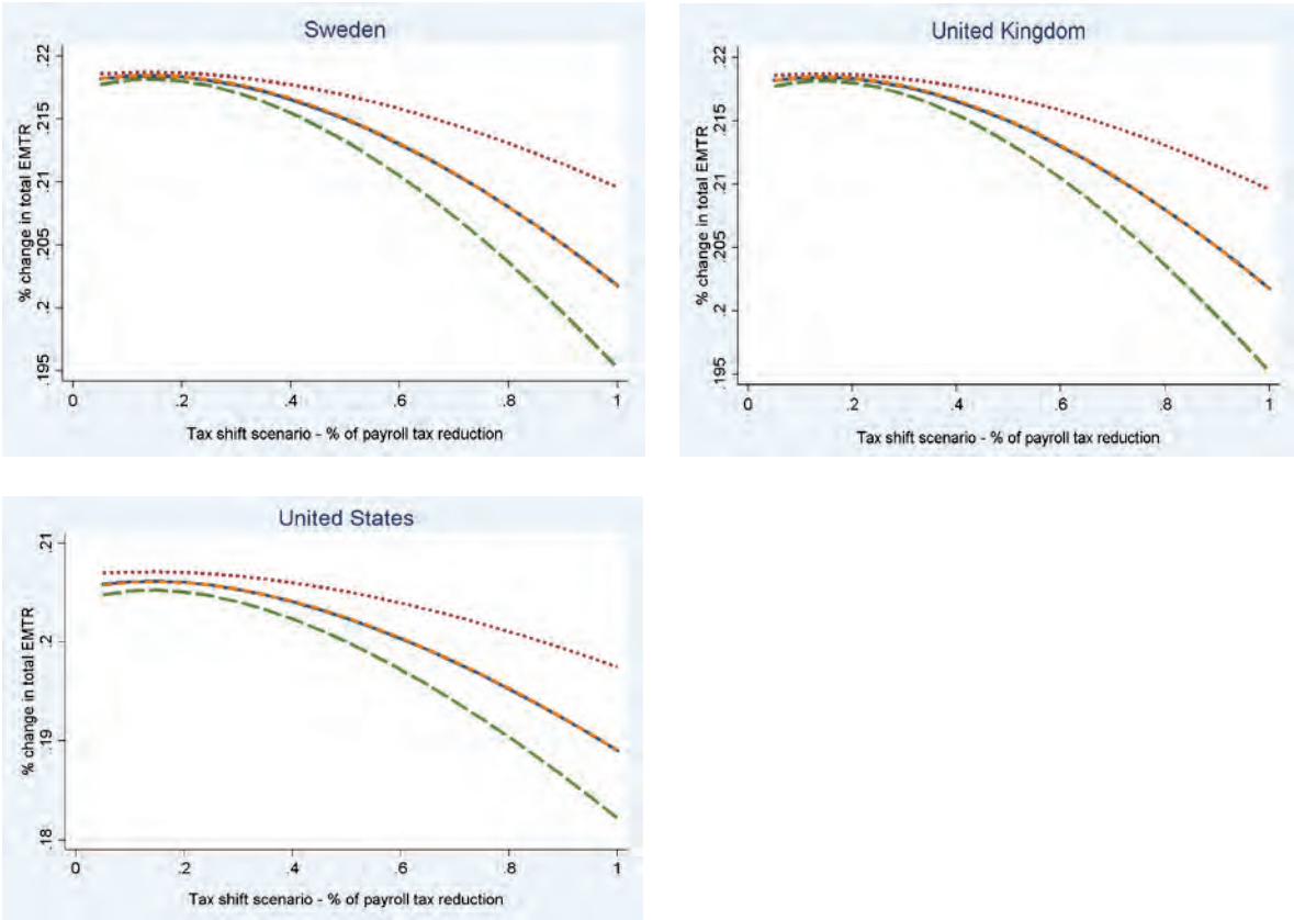
Figure (5) - continued: Labour to Energy Tax Shifting Simulation. (country-average results for 2010) – Results under alternative elasticity of substitution ( b ).
